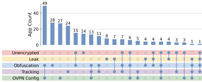
Fig. 4: Intersection of VPN app behaviors across the five analysis modules (traffic leaks, unencrypted content, VPN obfuscation, tracking/fingerprinting, and configuration issues).
